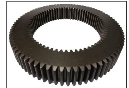
TR-01-0401-18 INTERNAL GEAR Z80-Z69
